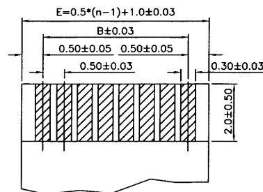
FFC/FPC DIMENSION
